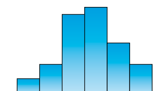
HISTOGRAMA
